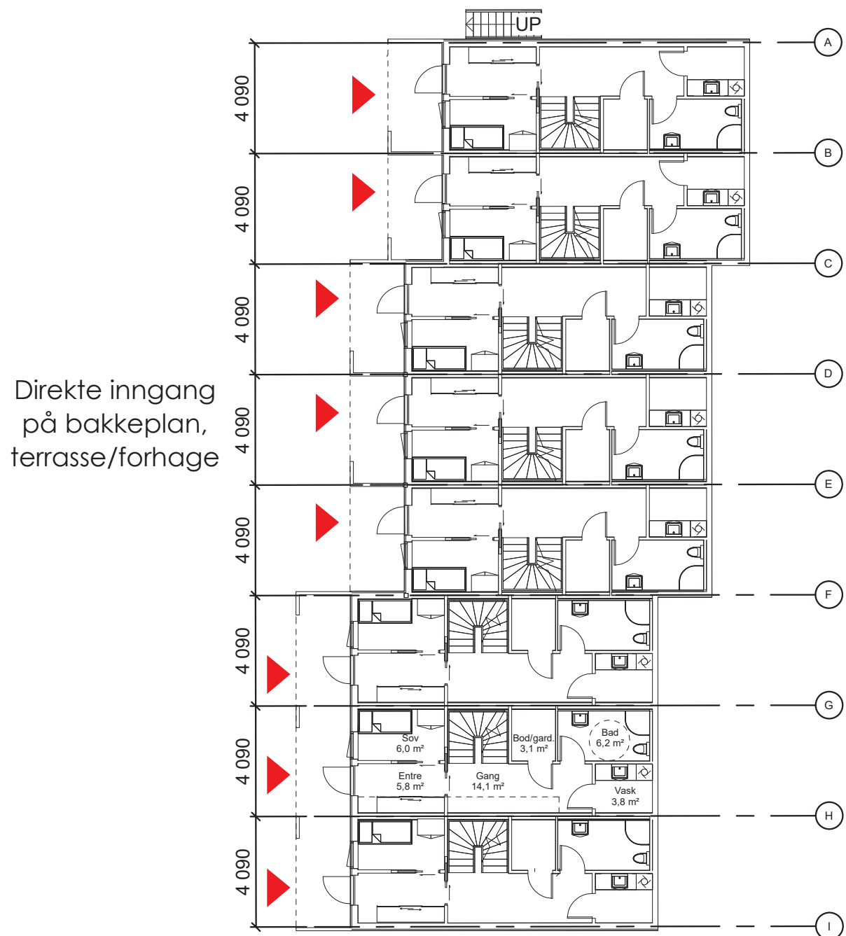
PLAN 1
